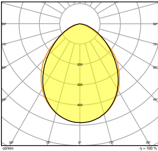
FL COMP SEN V S 20W 840 SYM 100 BK
